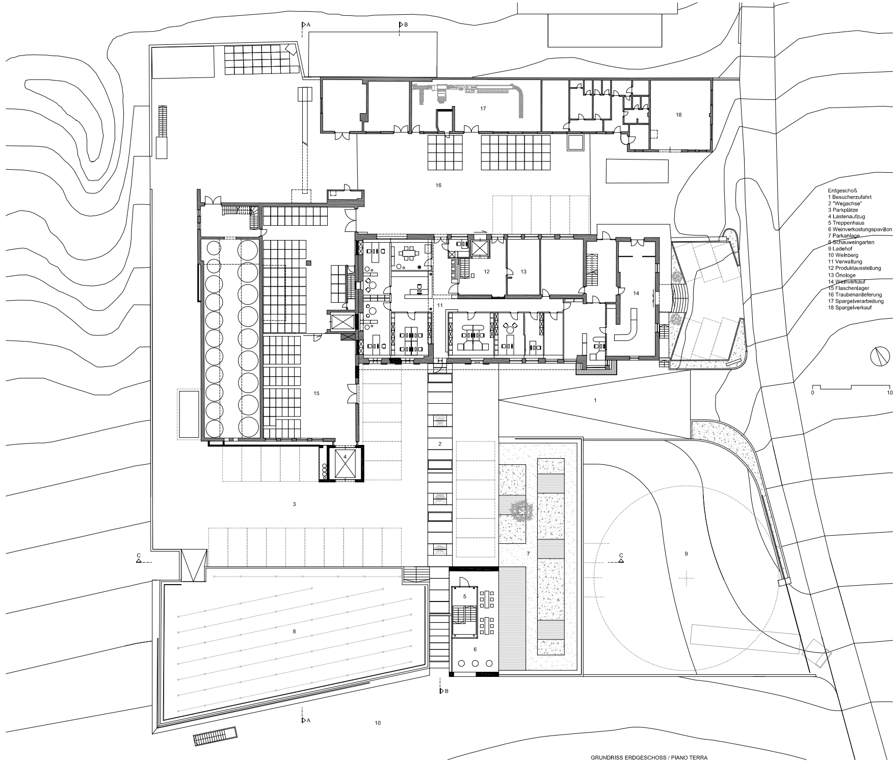
GRUNDRISS ERDGESCHOSS / PIANO TERRA
